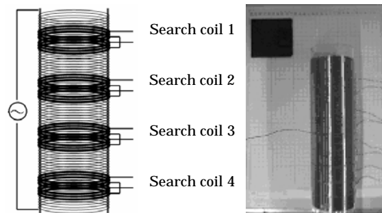
Fig.1 Schematic Diagram of the Tested Apparatus
