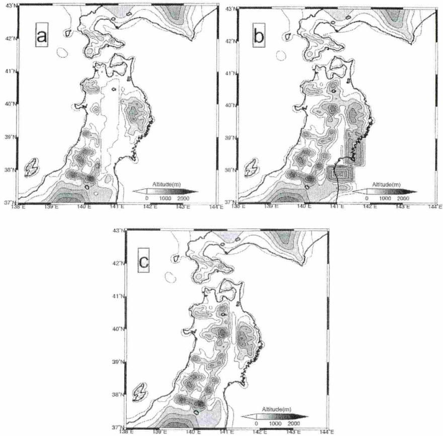
Fig. 8 Topography in numerical experiments assuming different topographic conditions (a: Removing Ou Mountains; b: blocking up Sendai Bay; c: connecting Kitakami Basin and Hachinohe)
