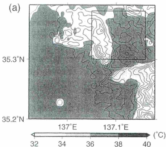
Fig. 9 Surface air temperature (shading) at 14:00 JST on August 18, 2010 in Tajimi and Kasugai from the WRF model control simulation (CTRL)
