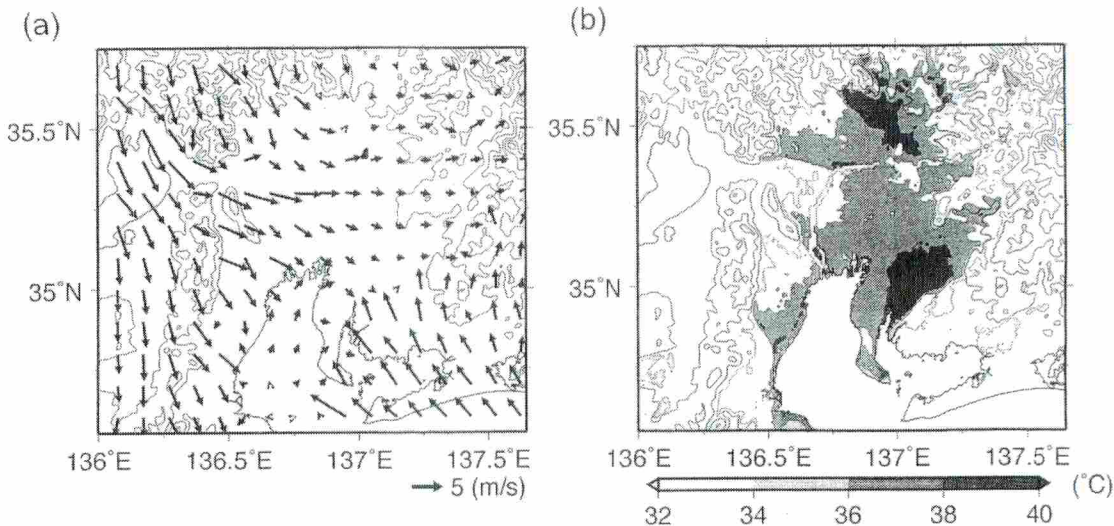
Fig. 8 (a) Wind field (vector) and (b) surface air temperature (shading) at 14:00 JST on August 18, 2010 from the WRF model control simulation (CTRL)
