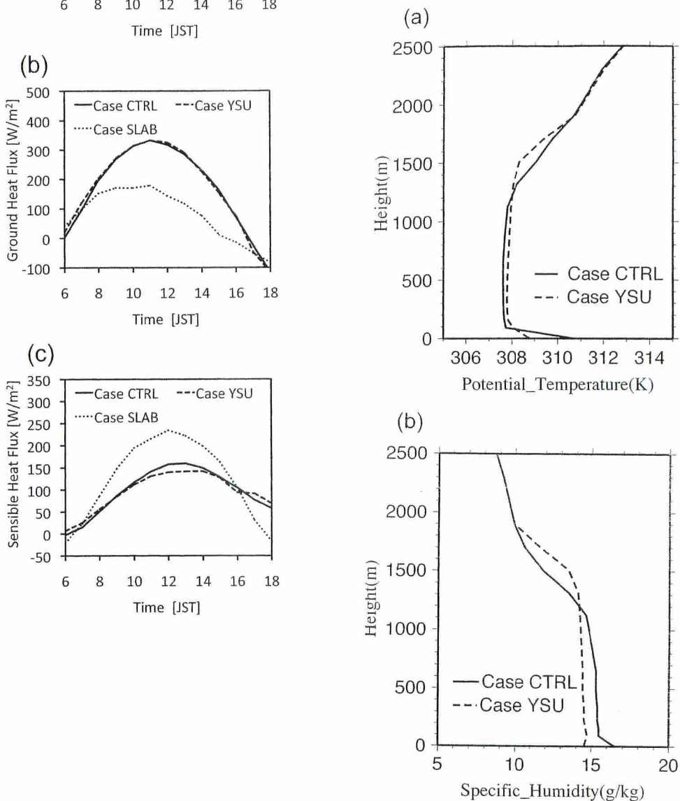
Fig. 14 Vertical profiles of (a) potential temperature and (b) specific humidity at 14:00 JST on August 18, 2010 in Taihei Park in Tajimi. The solid line indicates CTRL results, and the dashed line YSU results.
