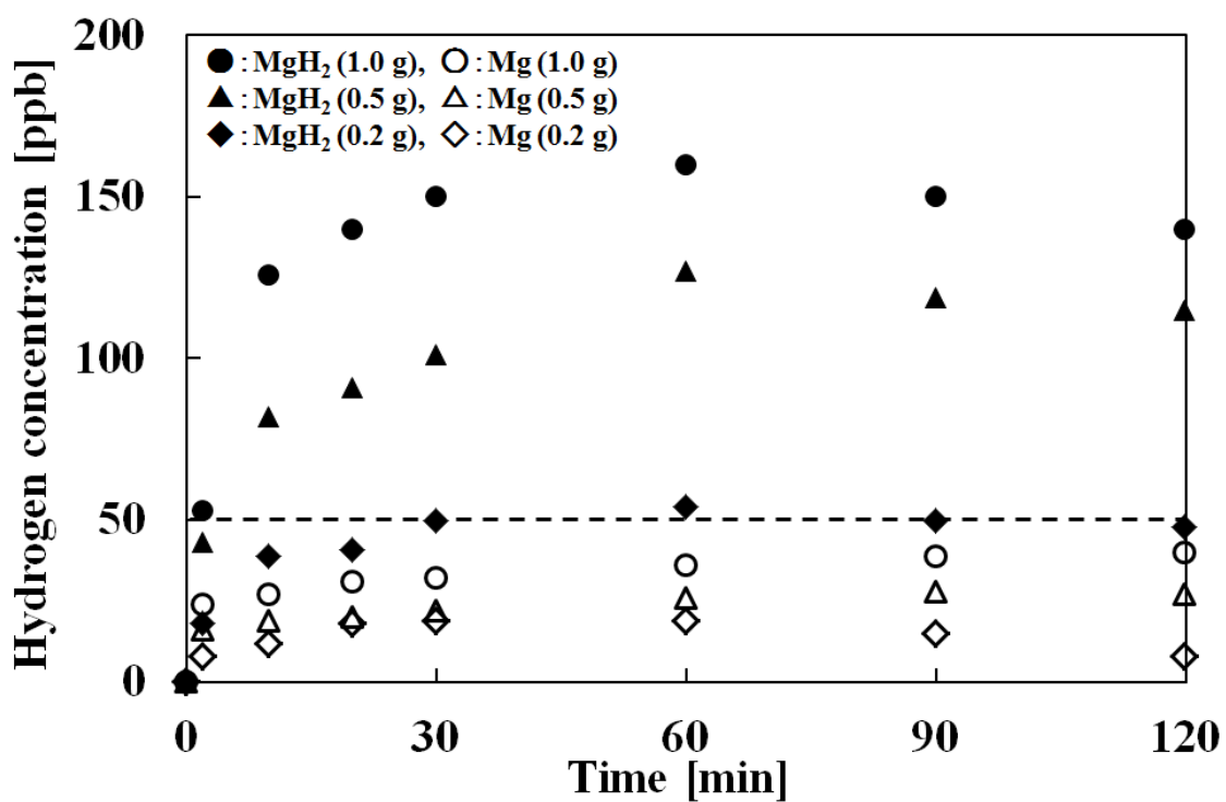
Fig.1.5 Changes in hydrogen concentration in bathwater by adding Mg and \text{MgH}_2 .
