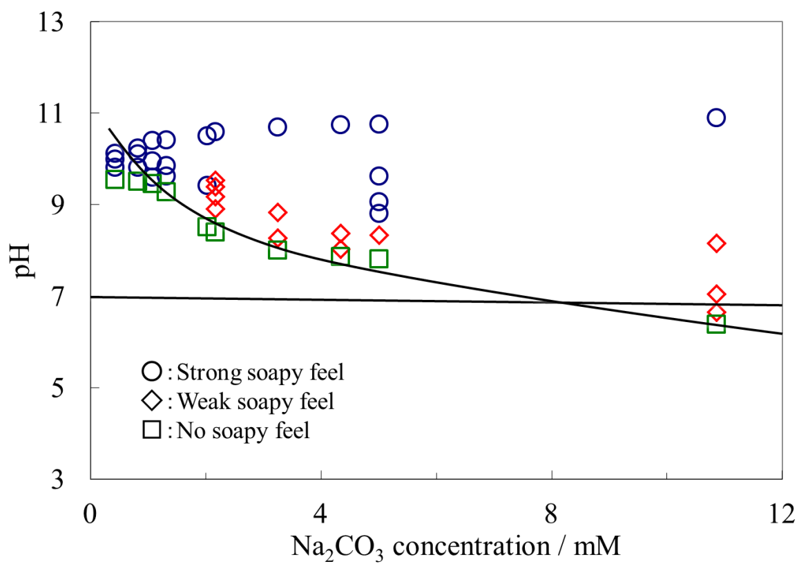
Fig. 1.4 The relationships between concentration and pH of \text{Na}_2\text{CO}_3 aqueous solution giving soapy feel to the skin in hydrochloric acid titration.
