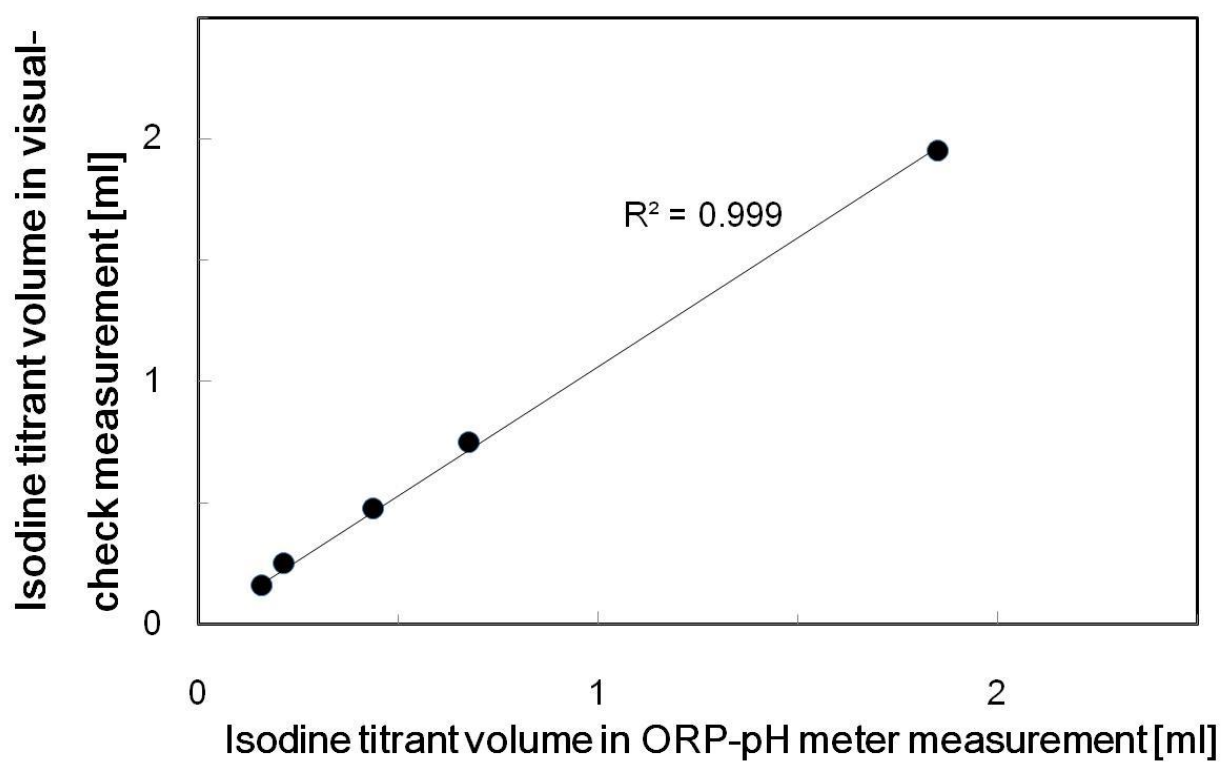
Fig. 1.3 Relationship in iodine (Isodine®) titrant volume between visual-check measurement and ORP-pH meter measurement in artificial sulfur spring waters.
