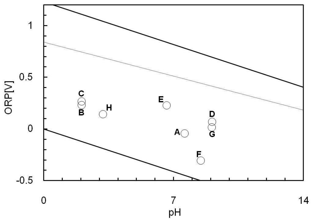
Fig. 1.6 ORP-pH relationship in samples of natural hot spring waters.
