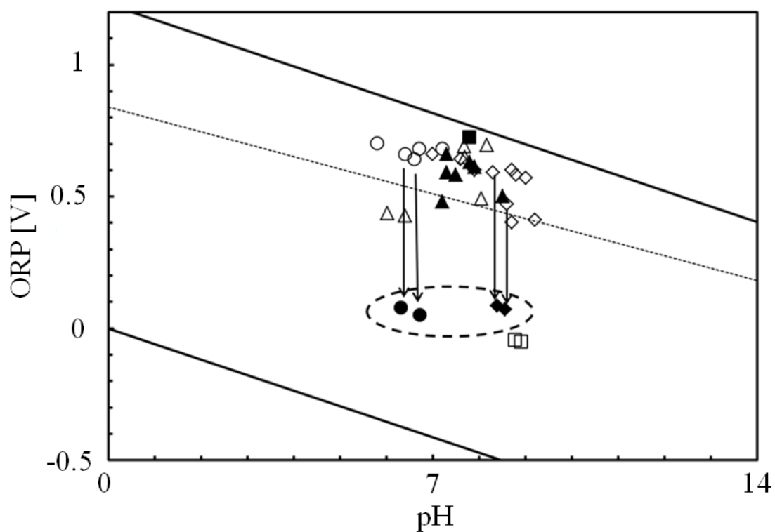
Fig.3.4 Changes in ORP-pH relationship of chlorinated tap water by adding mixtures of \text{MgH}_2 (1 g) and different commercial bath salts.
