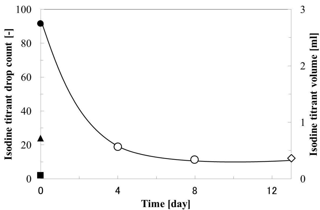
Fig. 2.3 Variation with time in Isodine® titrant volume in aging of fresh hot spring water.
