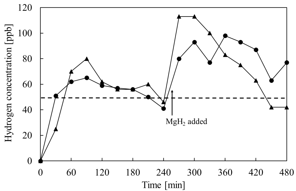
Fig.2.2 Changes with time in dissolved hydrogen concentration of hot spring water hydrogenated by addition of \text{MgH}_2 .
