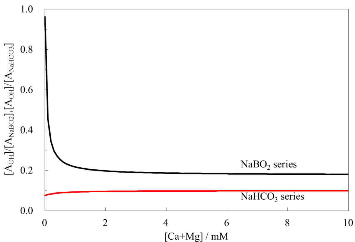
Fig. 1.9 Degree of contribution of NaBO 2 and NaHCO 3 series alkaline components in giving soapy feel to the skin with respect to NaOH series alkaline components under variations in [Ca+Mg] concentration.
