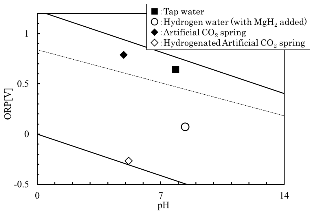
Fig.3.2 ORP-pH relationships of Hydrogenated Artificial \text{CO}_2 spring, Hydrogen water, Artificial \text{CO}_2 spring, and tap water.
