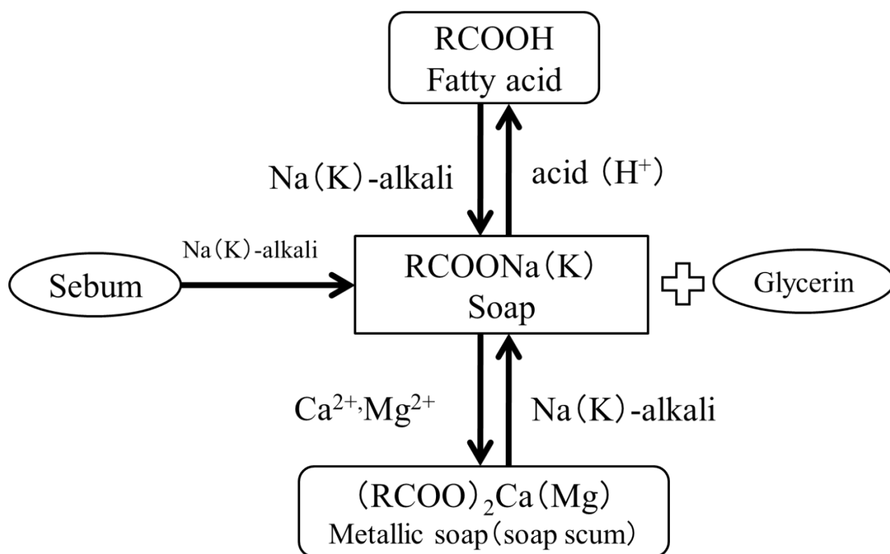
Fig. 1.1 The relationships of components of bathwater giving soapy feel to the skin.
