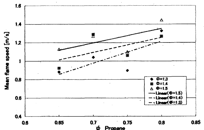
Fig. 5 Mean flame speed
