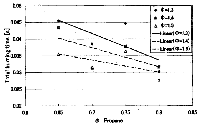
Fig. 4 Total burning time
