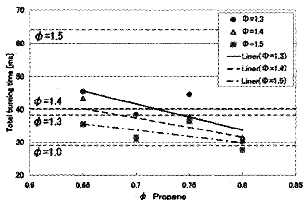
Fig.4 Total burning time (1 atm)
