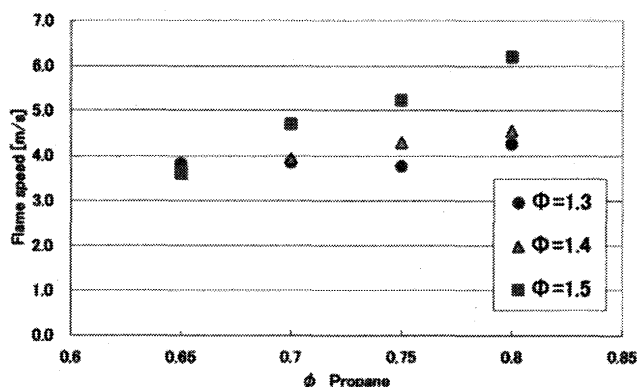
Fig.6 Flame speed (1 atm)
