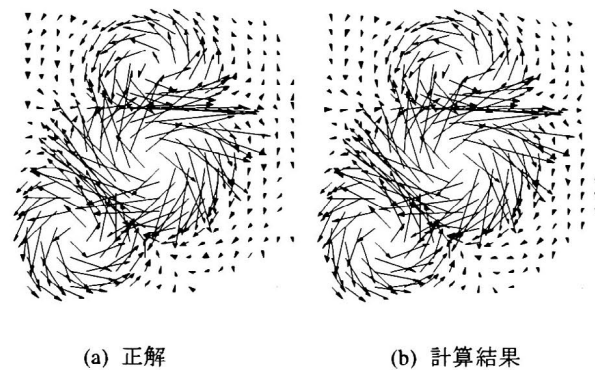
図 6. 電流ベクトル分布 Fig.6 Comparison (a) exact with (b) computed current vector distributions.
