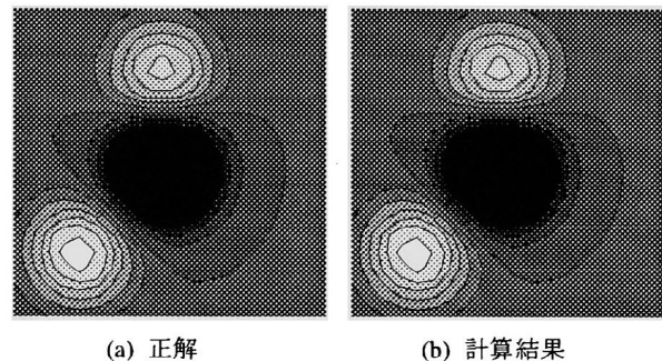
図 5. 電流分布 Fig.5 Comparison (a) exact with (b) computed current distributions.
