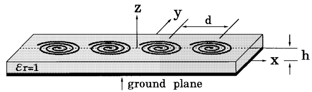
Fig. 9. An array composed of four monofilar spiral elements.
