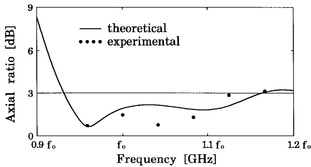
Fig. 7. Frequency response of the axial ratio in a direction of (\theta, \phi) = (\theta_{\max} = 28^\circ, \phi_{\max} = 232^\circ) .
