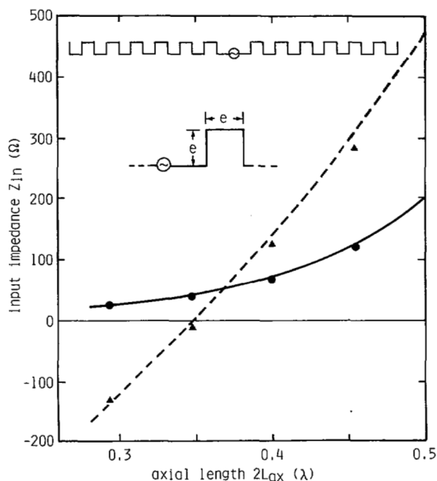
Fig. 5. Input impedance Z_{\text{in}} = R_{\text{in}} + jX_{\text{in}} of meander-line dipole antenna e = 0.0133 \lambda . Theoretical: R_{\text{in}} —, X_{\text{in}} ---. Experimental: R_{\text{in}} ●●, X_{\text{in}} ▲▲.
