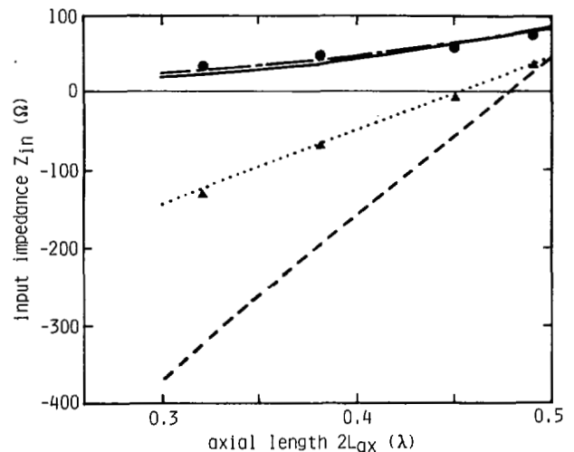
Fig. 2. Input impedance Z_{in} = R_{in} + jX_{in} . Linear dipole antenna, theoretical: R_{in} —, X_{in} - - -. Zigzag dipole antenna ( 2L_{wire} = 0.5\lambda , theoretical: R_{in} —, X_{in} - - -, experimental: R_{in} ●●, X_{in} ▲▲).
