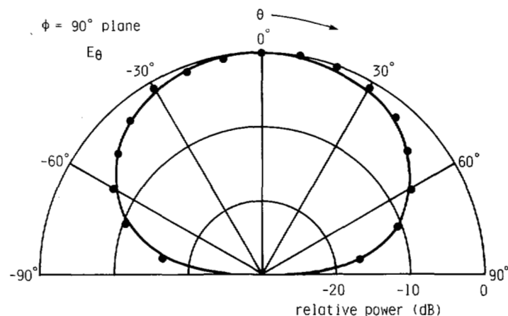
Fig. 3. Radiation pattern of zigzag dipole antenna ( 2L_{\text{wire}} = 0.5 \lambda , 2L_{\text{ax}} = 0.45 \lambda , \tau = 129^\circ ). Theoretical: —, Experimental: ●●.
