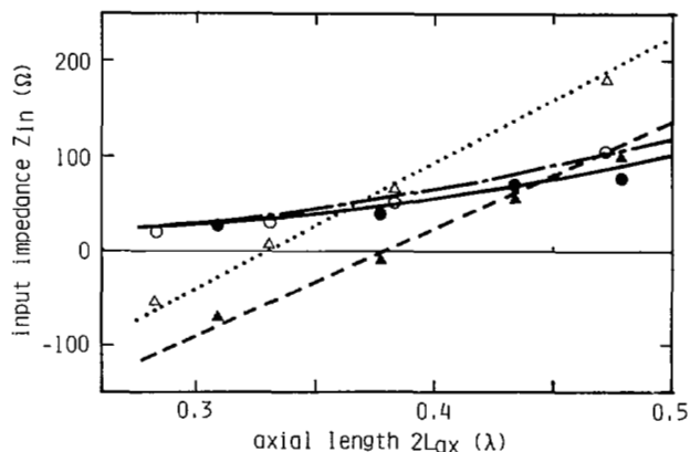
Fig. 4. Input impedance Z_{\text{in}} = R_{\text{in}} + jX_{\text{in}} of zigzag dipole antenna. 2L_{\text{wire}} = 0.58 \lambda , e_1 = e_8 = 0.0208 \lambda , e_2 = e_3 = \dots = e_7 = 0.0416 \lambda , theoretical: R_{\text{in}} —, X_{\text{in}} ---, experimental: R_{\text{in}} ●●, X_{\text{in}} ▲▲. 2L_{\text{wire}} = 0.67 \lambda , e_1 = e_9 = 0.0208 \lambda , e_2 = e_3 = \dots = e_8 = 0.0416 \lambda , theoretical: R_{\text{in}} —, X_{\text{in}} ---, experimental: R_{\text{in}} ○○, X_{\text{in}} △△.
