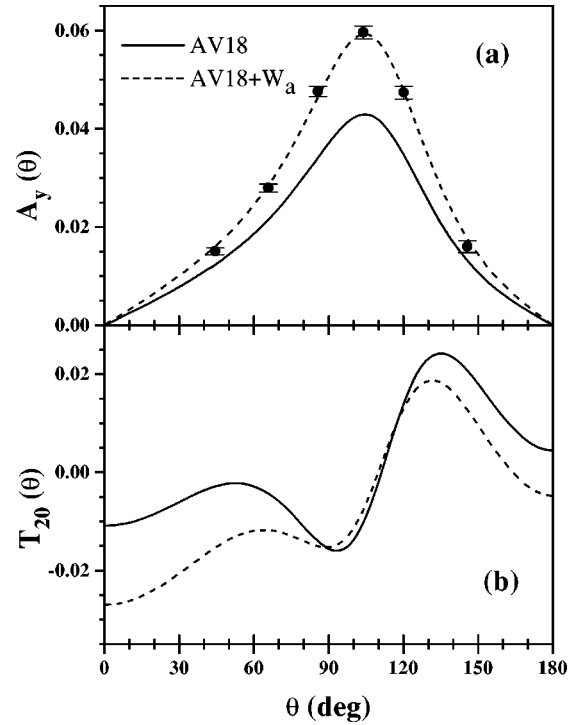
FIG. 2. A_y(\theta) at E_{\text{Lab}}^n=3 MeV (a) and T_{20}(\theta) at E_{\text{Lab}}^d=6 MeV (b) calculated with AV18 (solid lines) and AV18+ W_a (dashed lines). Experimental data of A_y(\theta) are taken from Ref. [4].
