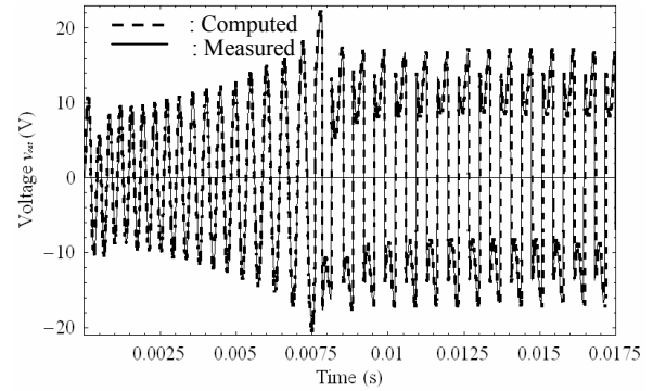
Fig.6 Calculated voltage V_{out} vs. time t .
