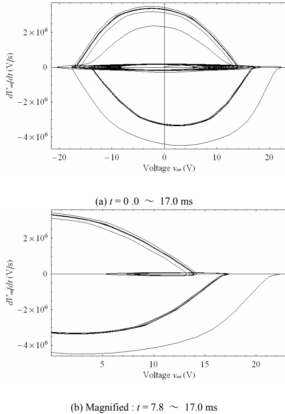
Fig. 7 Trajectory of dV_{out}/dt vs. V_{out} exhibiting a chaotic behavior.
