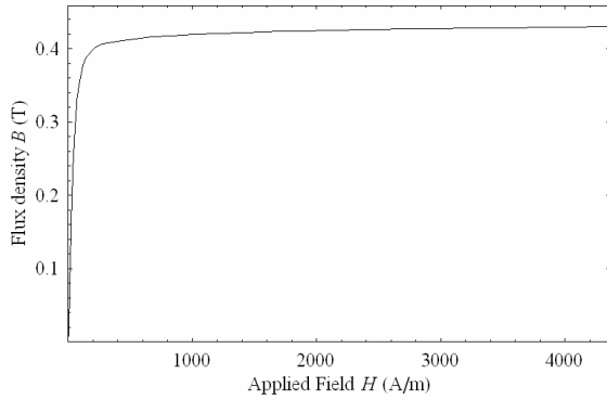
Fig. 1 Magnetization Curve Giving Permeability \mu (TDK H5A).
