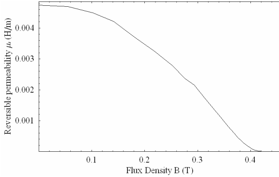
Fig. 2 Reversible Permeability \mu_r (TDK H5A).
