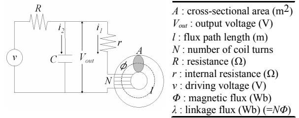
Fig. 4 Parallel Ferroresonant Circuit.
